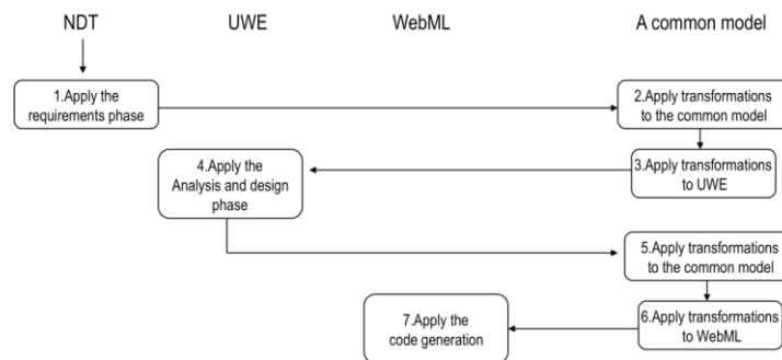
FIGURE 2. Use of common metamodels to make approaches compatible
