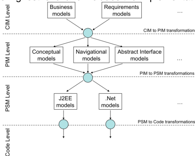
FIGURE 3. MDA structure for Web engineering (based on [43]).
